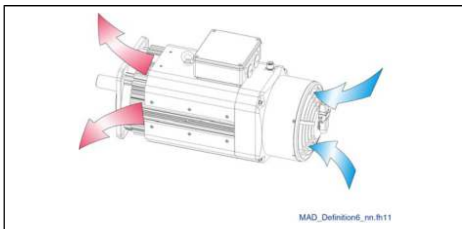
Fig.6-1: MAD, blowing axial fan
