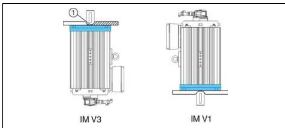
Fig.9-10: Example: vertical MAF installation position
