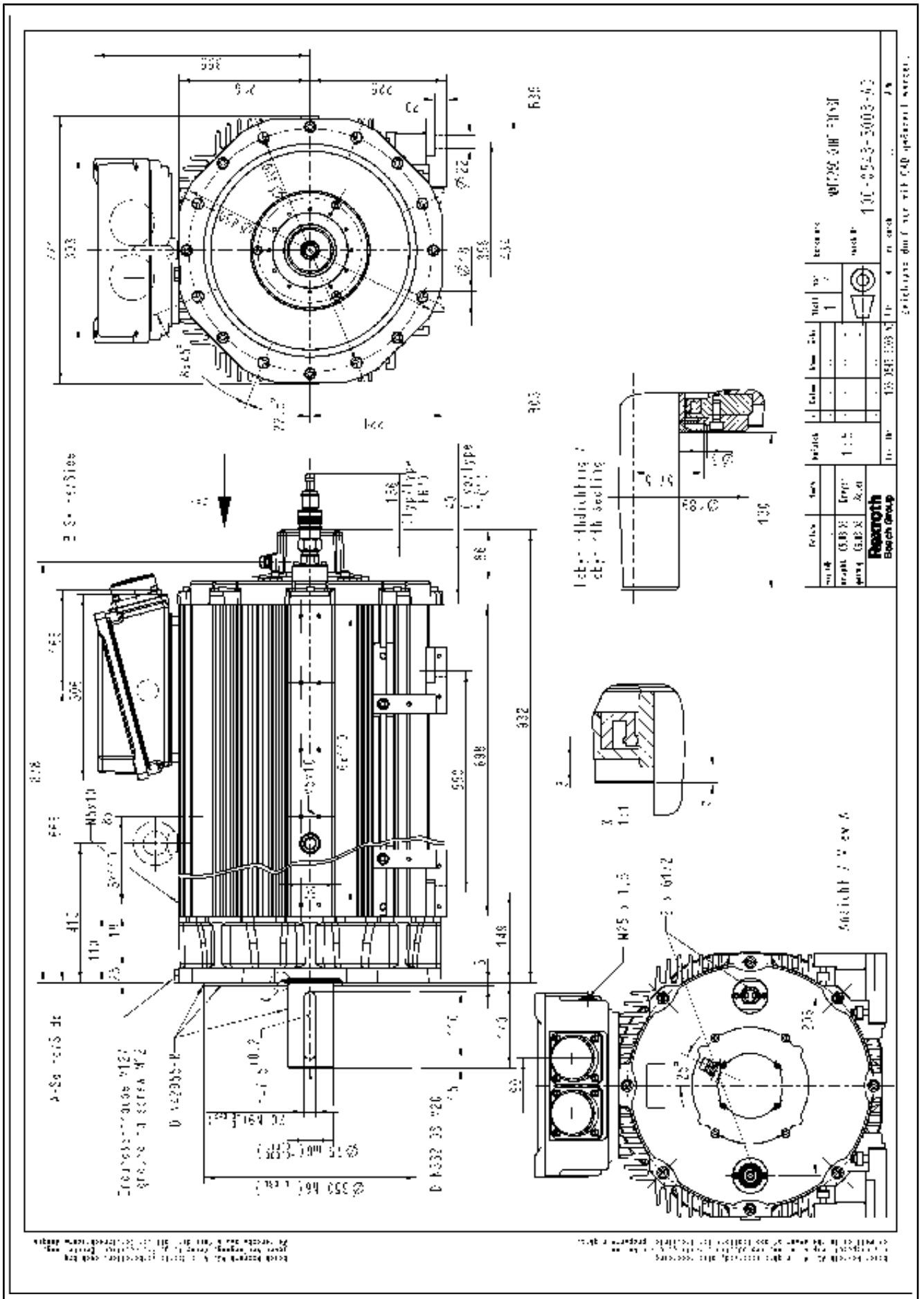
Fig.5-48: MAF225C without brake
