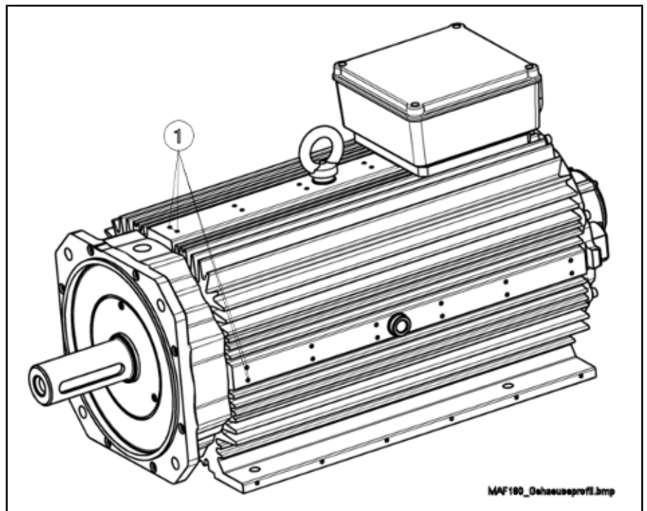
① M5 threaded holes
