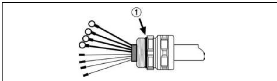
① O-ring position
