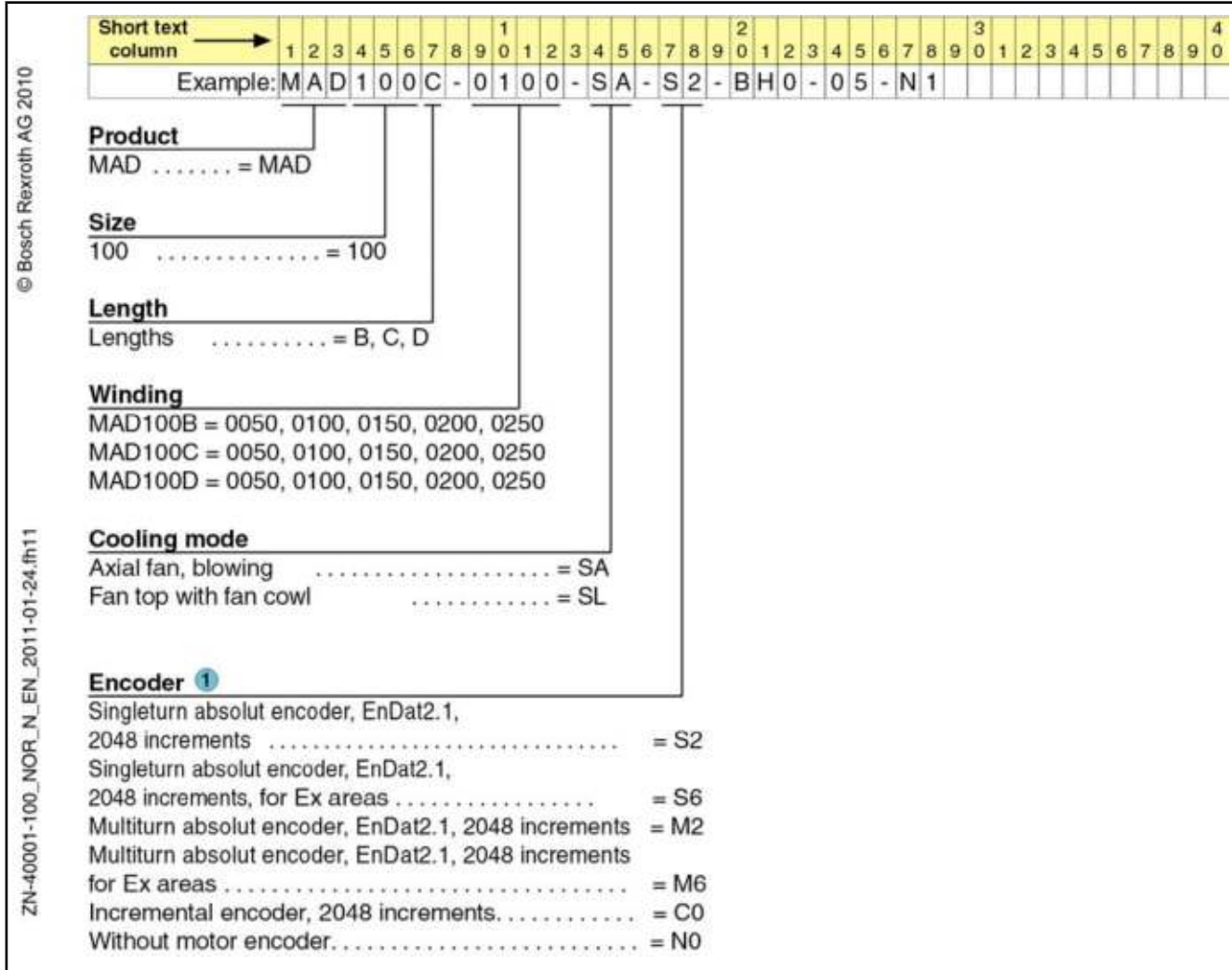
Fig.6-4: Type code MAD100 (1/2)
