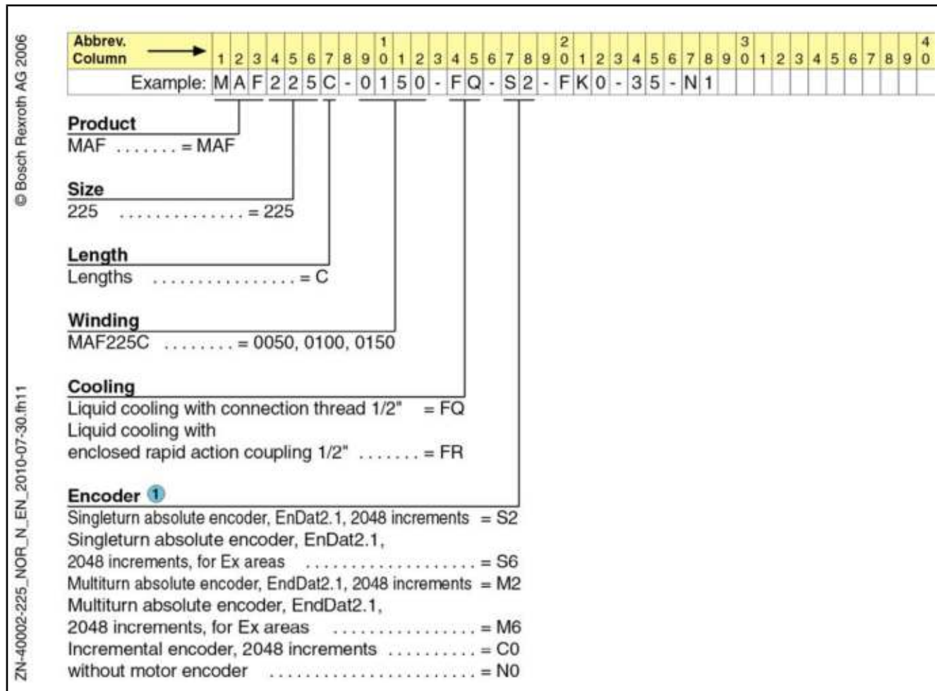
Fig.6-22: Type code MAF225 (1/2)
